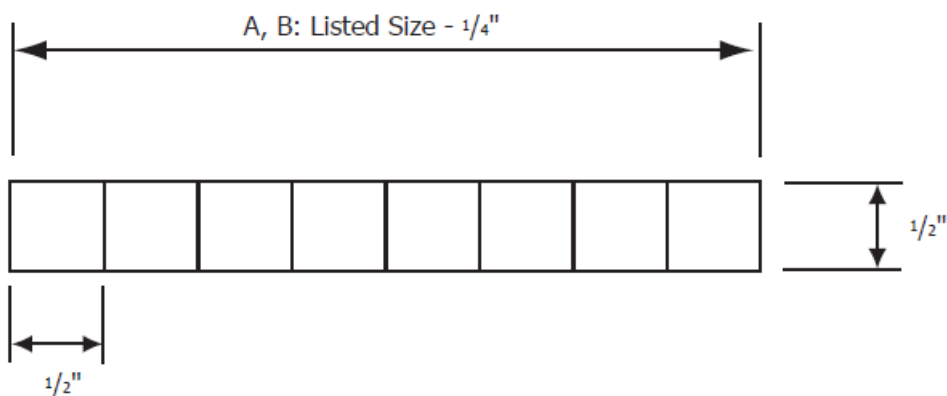
ERN Aluminum Grid Core
